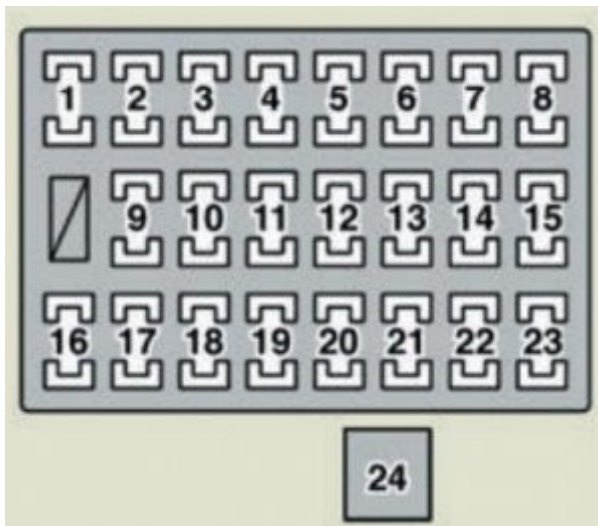
Lexus GX470 – fuse box –
